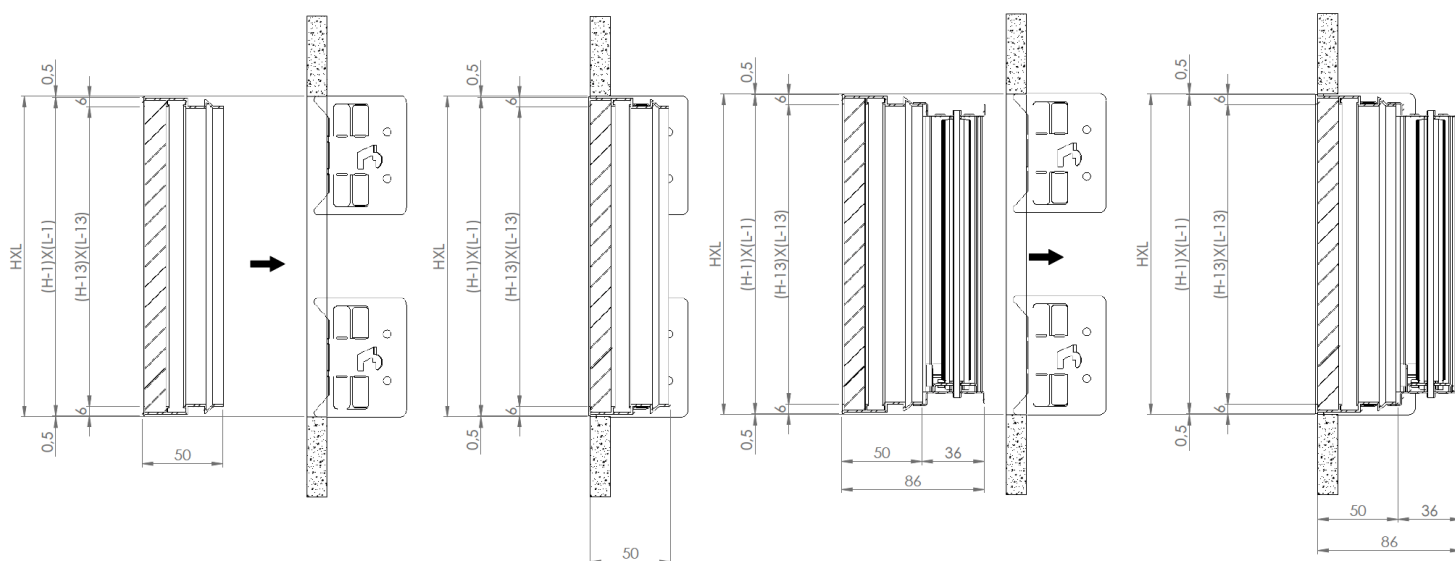
SC - Regulation damper
