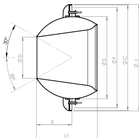
EDU EDU/M senza coprighiera EDU EDU/M without screw cover
