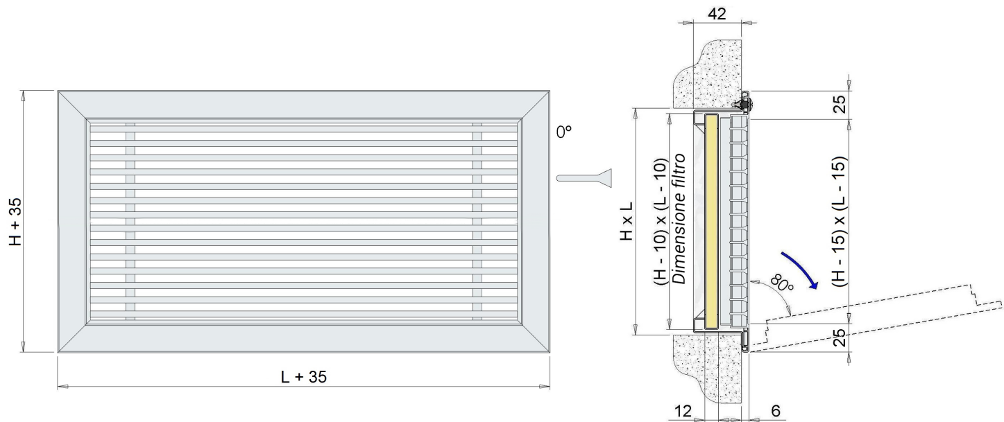
EBL3 20/0° DIMENSIONI FRONTALI FRONTAL DIMENSIONS EBL3 20/0°
